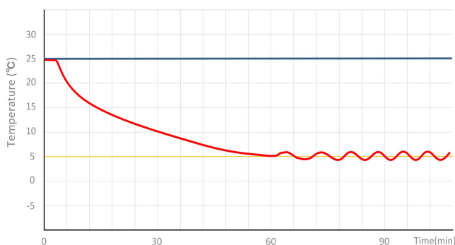
YR05087-1 PULL DOWN TEST
